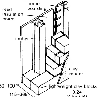
⑩ Balloon frame with lightweight clay blocks 0.24 W/(m 2 ·K)
